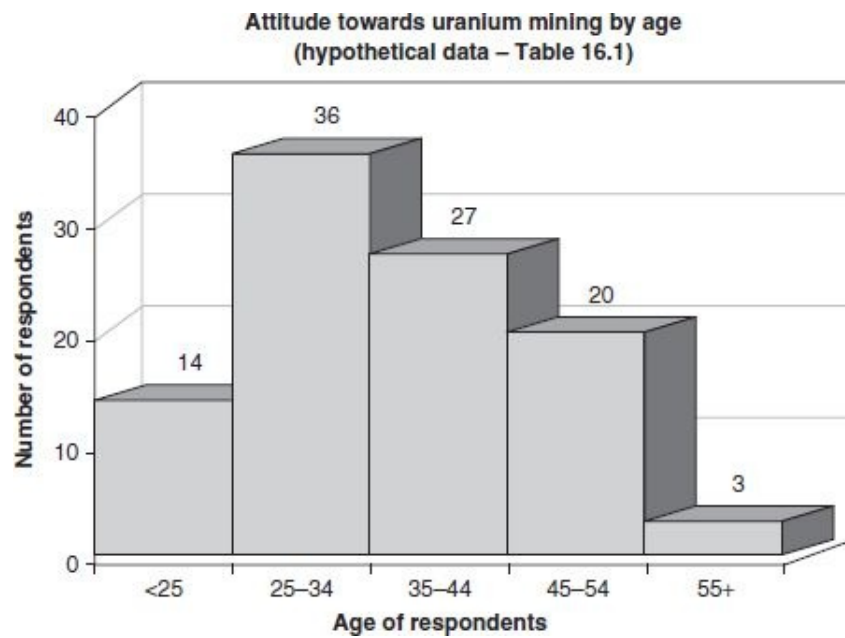
FIGURE 16.2b Three-dimensional histogram
