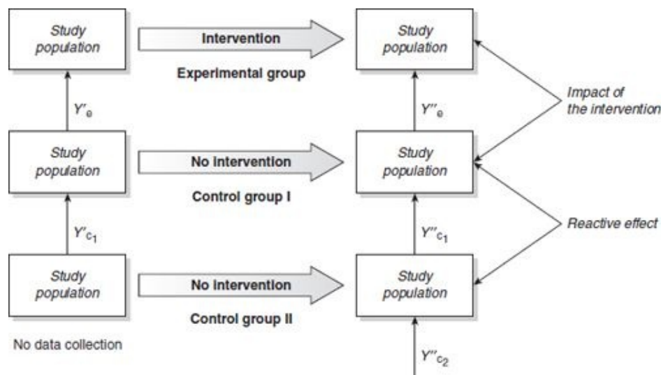
FIGURE 8.11 Double-control designs
