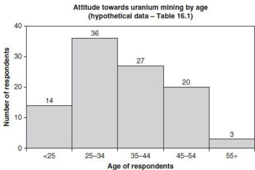
FIGURE 16.2a Two-dimensional histogram
