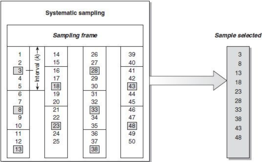
FIGURE 12.9 Systematic sampling
