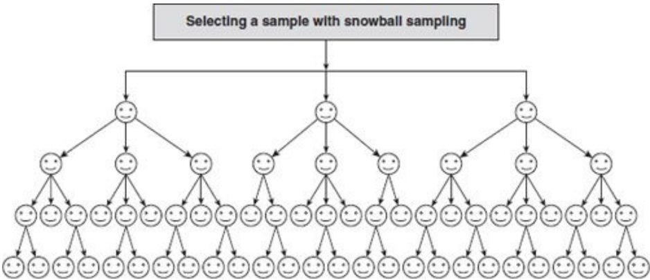
FIGURE 12.7 Snowball sampling
